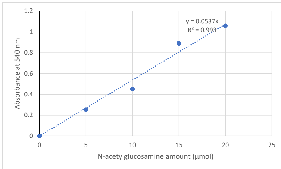
Figure C: Standard curve of N-acetylglucosamine
